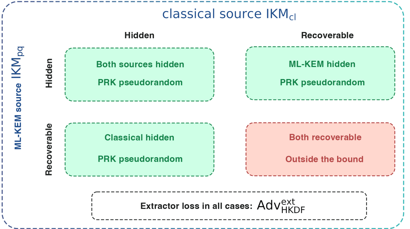
Figure 5. Condition map for the hybrid-combiner interpretation used in Eq. (23). Rows and columns describe whether the classical or ML-KEM source remains hidden relative to a fixed transcript. Under the concatenation-combiner interpretation, the PRK remains pseudorandom whenever at least one source remains hidden. Simultaneous recovery of both sources is the source-level condition not ruled out by the bound, up to the additive Adv_{HKDF}^{skPRF} term.
